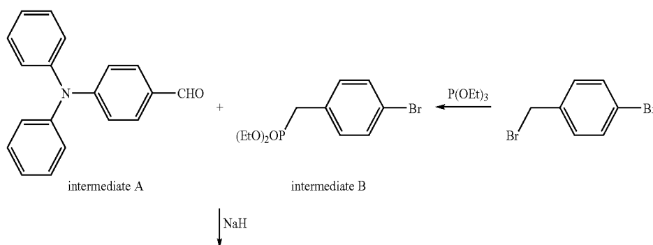
Reaction Scheme 2
