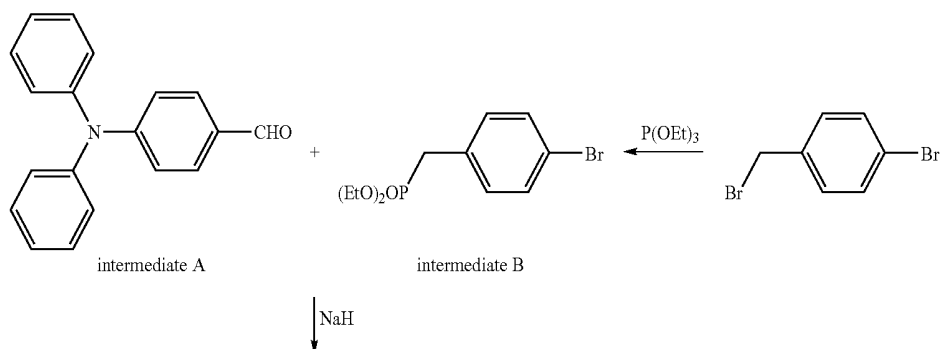
Reaction Scheme 3
